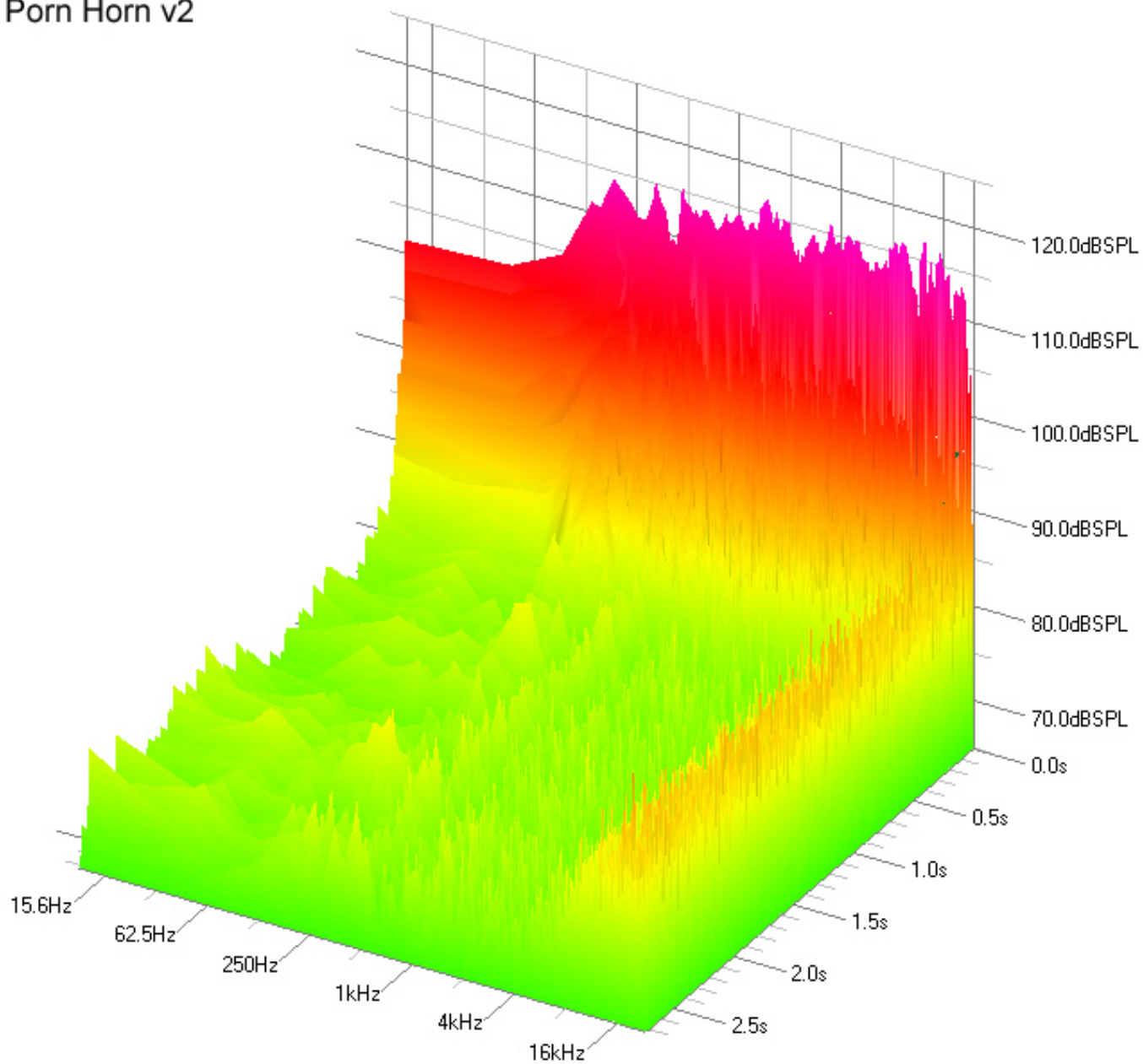
Impulse Response (Full IR) Porn Horn v2
